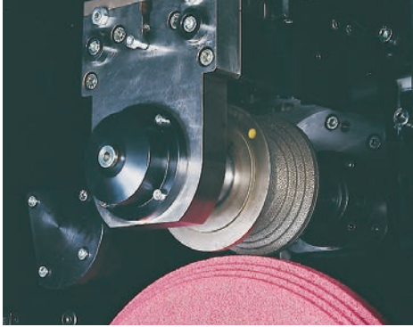
SinglespindleCD-dressingsystemmounted on wheel hand (V-axis)
