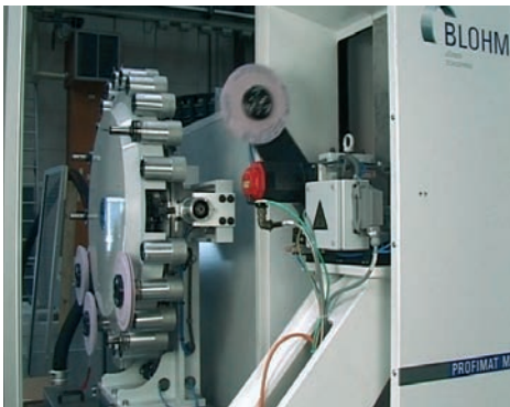
Tool changing systems with up to 24 tools 12 x D=300 or 8 x D=400
