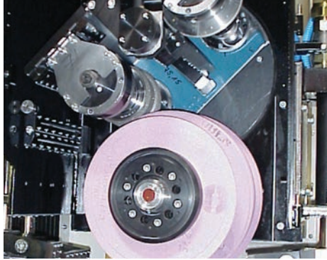
DoublespindleCD-dressingsystemmounted on wheel head (E-axis)
