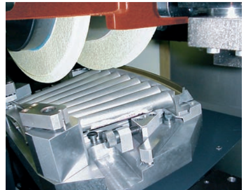
Turbine vane segment (MC 607 VG)
