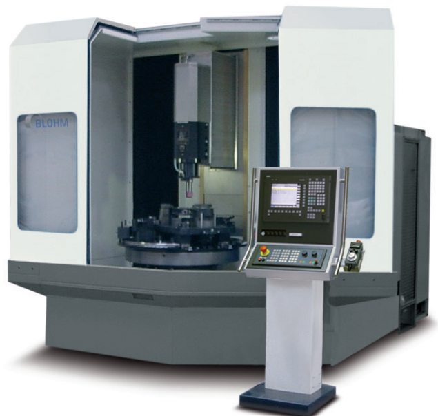
PROFIMAT MC 610VS with vertical grinding spindle
