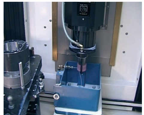
CNC dressing with single point diamond
